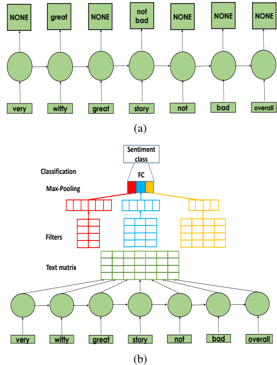
Figure 2: The PBLM model (figure imported from ZR18). (a) The PBLM representation learning model. (b) Adapting a classifier with PBLM: the PBLM-CNN model where PBLM representations are fed into a CNN task classifier.
