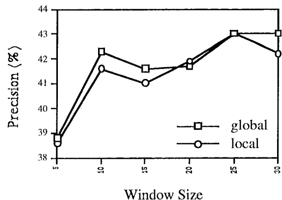
Figure 4: local nhyp vs. global nhyp
