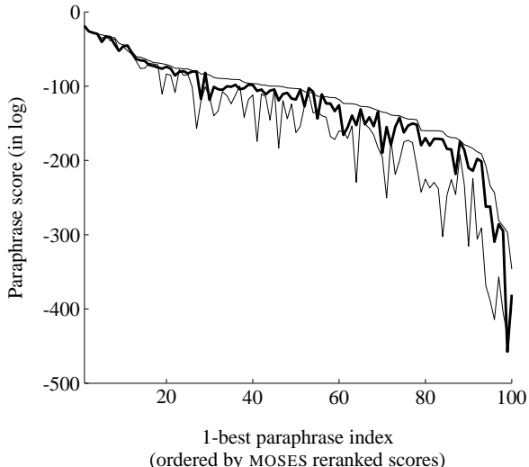
Figure 3: Comparison of paraphrase generators. Top: the MOSES baseline; middle and bold: the “true-score” MCPG; down: the “translator” MCPG. The use of “true-score” improves the MCPG performances. MCPG reaches MOSES performance level.
