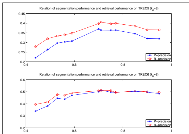
Figure 4: Results for k_d = 8 .
