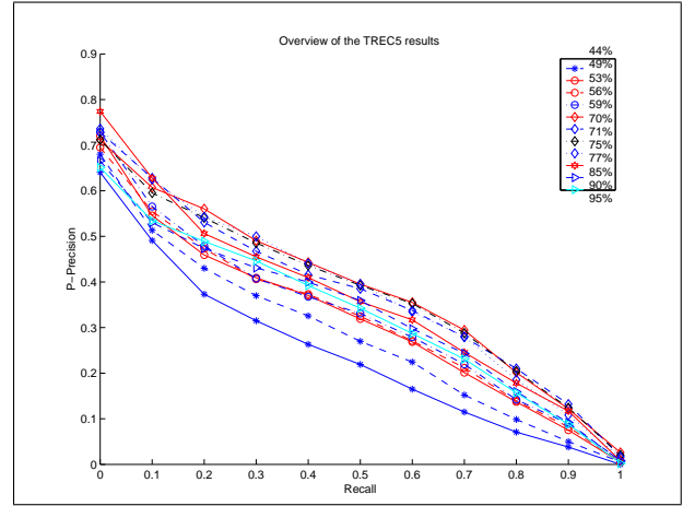
Figure 8: TREC5 precision-recall comprehensive view at k_d = 10
