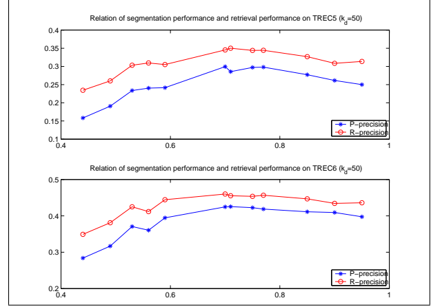
Figure 7: Results for k_d = 50 .
