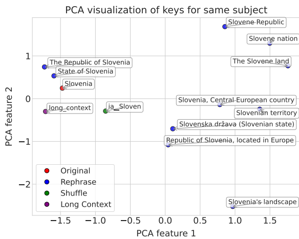
Figure 7: A visualization for key representations of rephrases for 'Slovenia' in LLaMA2-7B.
