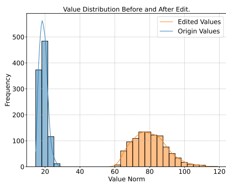
Figure 8: Values before and after edit with ROME.
