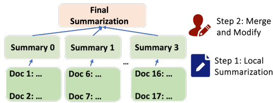
Figure 8: HierSphere for multi-faceted summarization.
