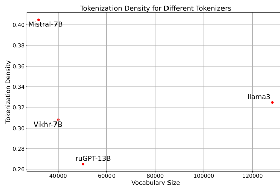
Figure 1: The efficiency of the Vikhr tokenizer for Russian in comparison to tokenizers of other models.
