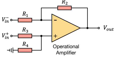
Figure 3: The operational amplifier with two input voltages V_{in}^+ and V_{in}^- . The CMRR \mathcal{K} is controlled by resistances R_1, R_2, R_3, R_4 .
