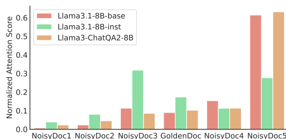
Figure 1: Normalized attention score. Transformers often miss the golden document in a noisy context.
