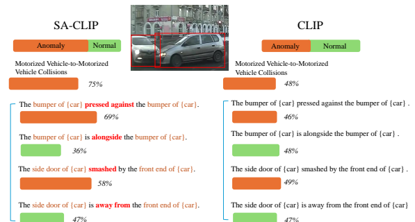
Figure 1: Comparison of image-text matching scores between SA-CLIP and CLIP in the traffic anomaly scene. SA-CLIP focuses on the objects and relationships between the objects both in image and text, and achieves better anomaly detection ability than the vanilla CLIP.
