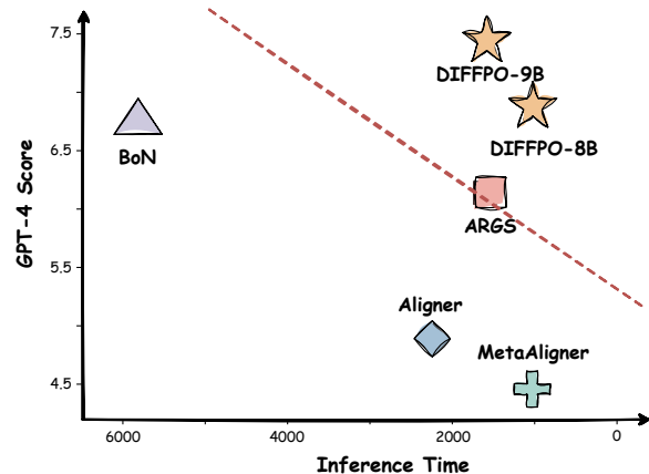
Figure 1: Comparison with Inference-Time Methods. Points closer to the top-right indicate a superior trade-off between performance and inference time.
