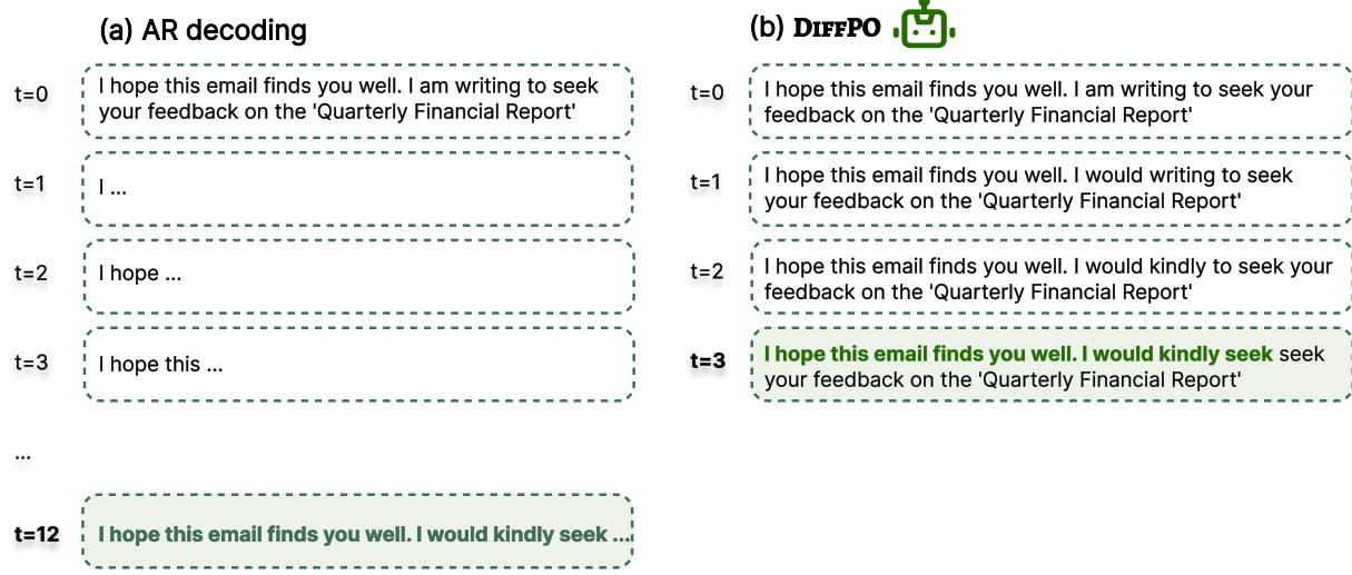
Figure 4: Illustration of the Speedup of DIFFPO.
