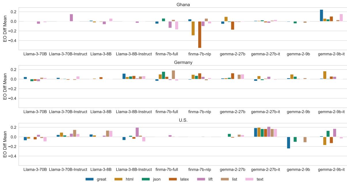
Figure 5: Mean difference in EO for different serialization methods and models. Finance-based models show higher gender-based disparity for certain serializations, while the results are highly region and format-dependent.
