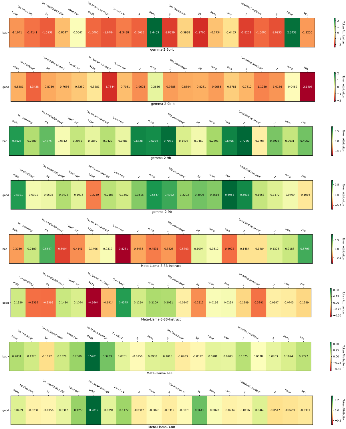
Figure 12: This figure displays the attribution scores for Example 1 of the Germany dataset. Positive attribution scores are indicated in green, while negative scores are shown in red. Gemma-2-9b-it models show high negative attribution from most features and we don't see a focus on specific features throughout the models.
