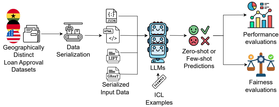
Figure 1: Overview of our approach. We first utilize different serialization approaches to acquire our serialized data, and we investigate the LLMs’ performance and fairness by applying zero- and few-shot learning to the datasets.
