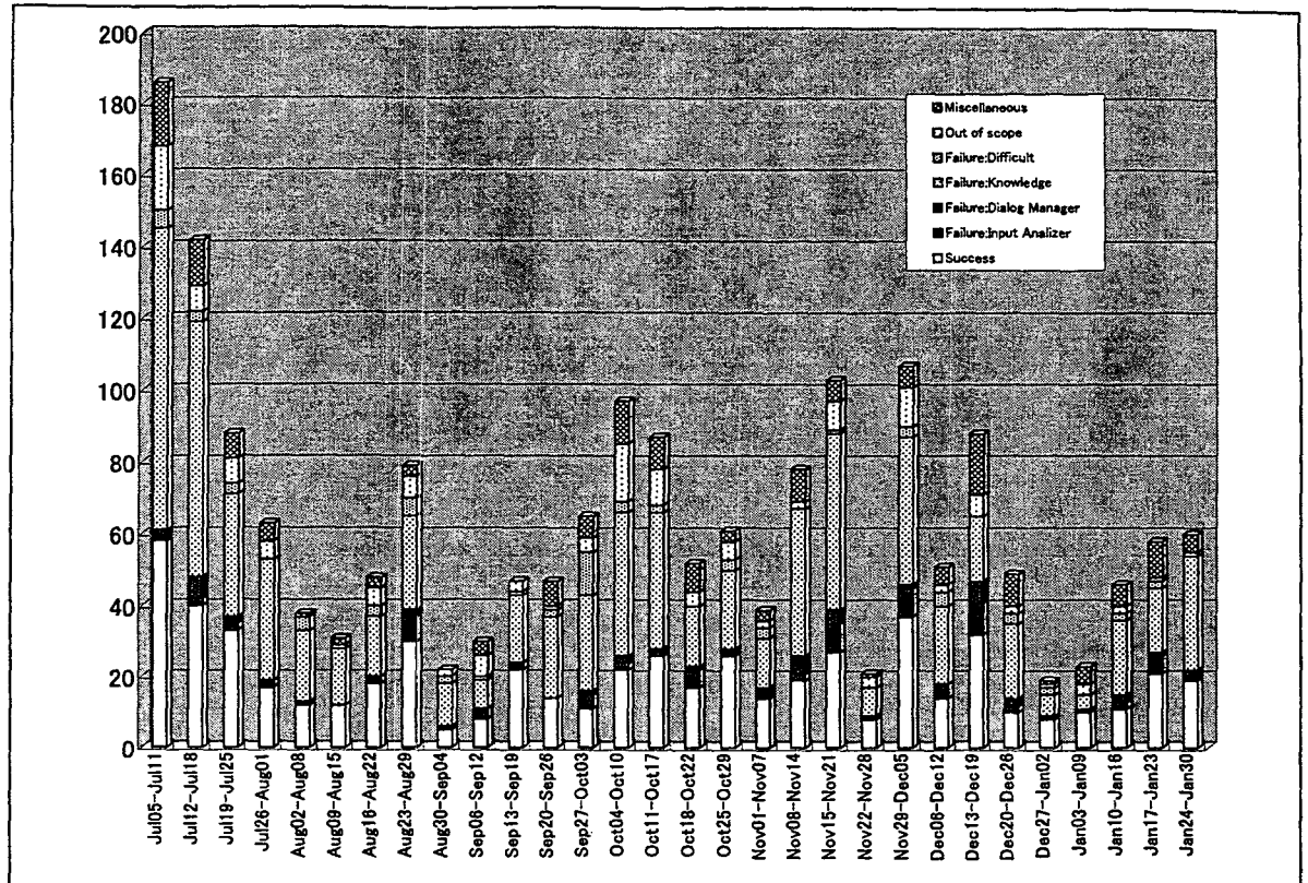
Figure 4: Evaluation of the helpsystem.
