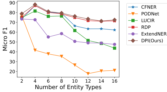
Figure 5: Task-wise results on the I2B2 (Murphy et al., 2010) dataset.
