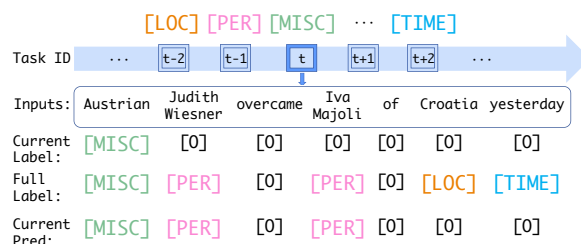
Figure 1: Challenges in INER. At the current incremental step t , the data is only annotated with the current entity type [MISC], while previous entity types [LOC] and [PER] are annotated with [O]. [TIME] is a future entity type. “Current Pred” indicates that the model forgets previous entity type [LOC] after step t .
