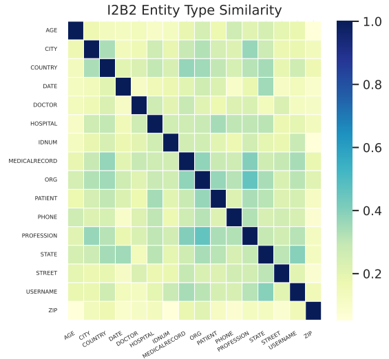
Figure 7: Entity type similarity of the I2B2 (Murphy et al., 2010) dataset.
