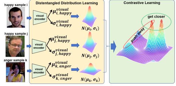
Figure 3: In the latent emotion space, we decouple emotion-related, modality-specific samples into separate distributions and use CL to group samples of the same category together while separating samples from different categories.
