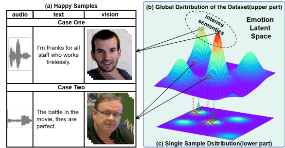
Figure 1: An illustration of aleatoric uncertainty in MMER task. When adopting Gaussian distribution modeling in latent emotion space, case two's semantic feature is more fuzzed with a larger variance due to cold speaking style than case one. Meanwhile, case one has stronger emotion intense located closer to the center of global distribution.
