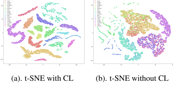
Figure 4: The t-SNE visualization of embedding with /without CL datasets. Different colors represent different label-related modality-special features of samples.
