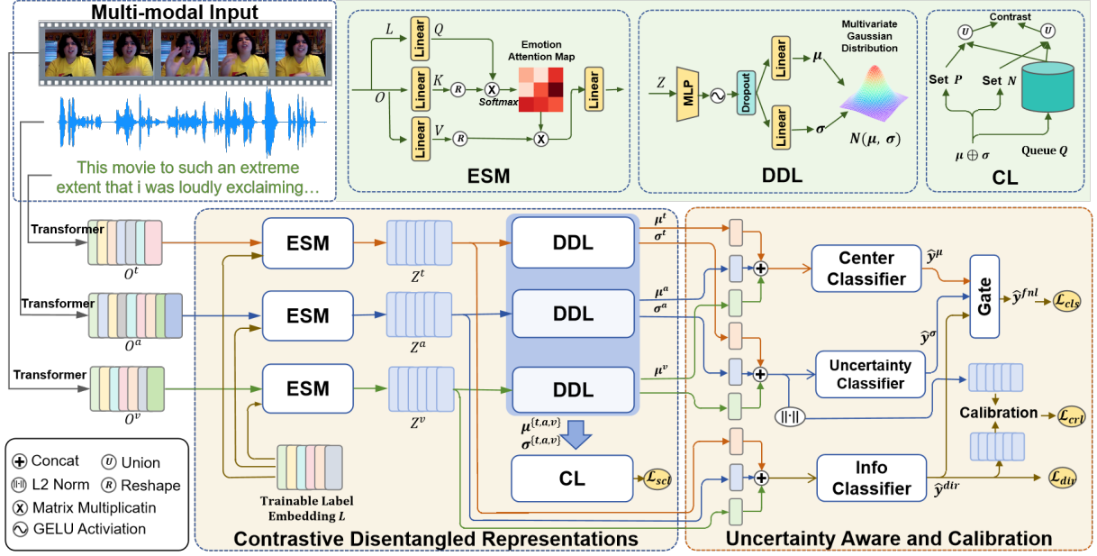
Figure 2: The proposed LDDU framework consists of three components: (1) the transformer-base unimodal extractor (2) a contrastive learning-based emotion space decomposition module, and (3) an uncertainty-aware fusion and uncertainty calibration module.
