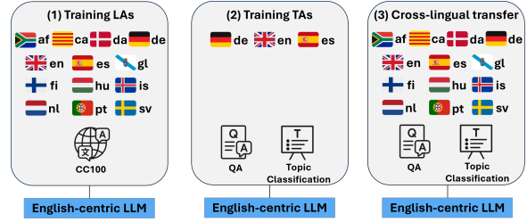
Figure 1: To evaluate cross-lingual transfer, language adapters (for 13 languages) and task adapters (for 3 high-resource source languages) are trained on top of a frozen English-centric LLM. Task adapters are evaluated on all languages of interest on two selected tasks.
