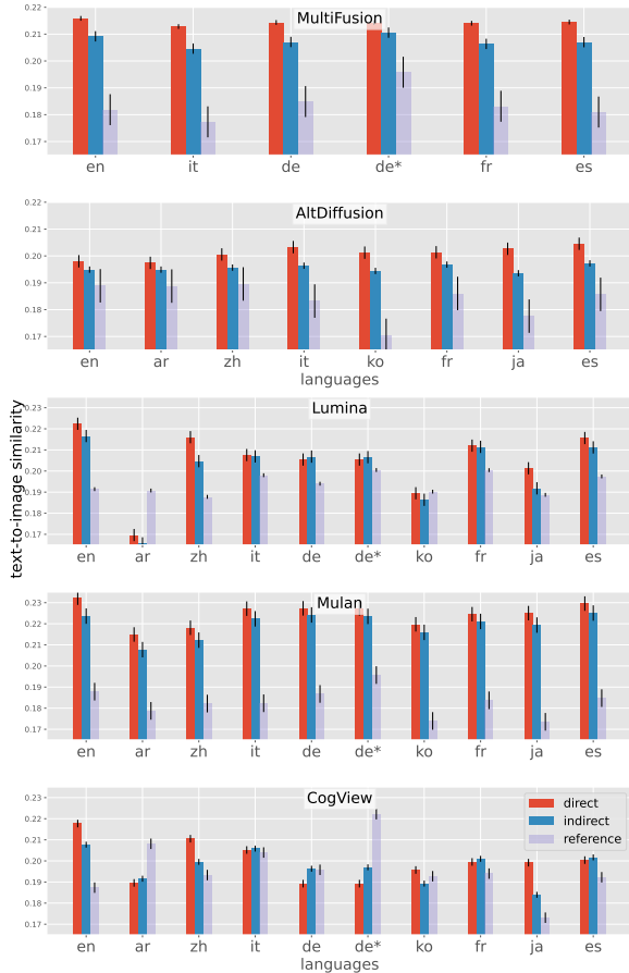
Figure 6: Text-to-image alignment for all models across languages. Red is direct-text-to-direct-images and blue is direct-text-to-indirect-images. Purple is the reference prompt t_r , “a photo of the face of a person”. Direct prompts align better with generated images than indirect prompts, indicating that bias reduction through prompt engineering affects alignment.
