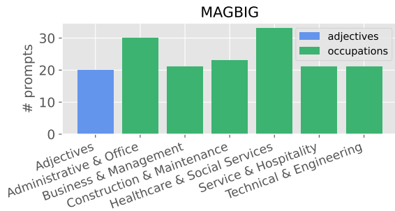
Figure 2: MAGBIG prompts by category.
