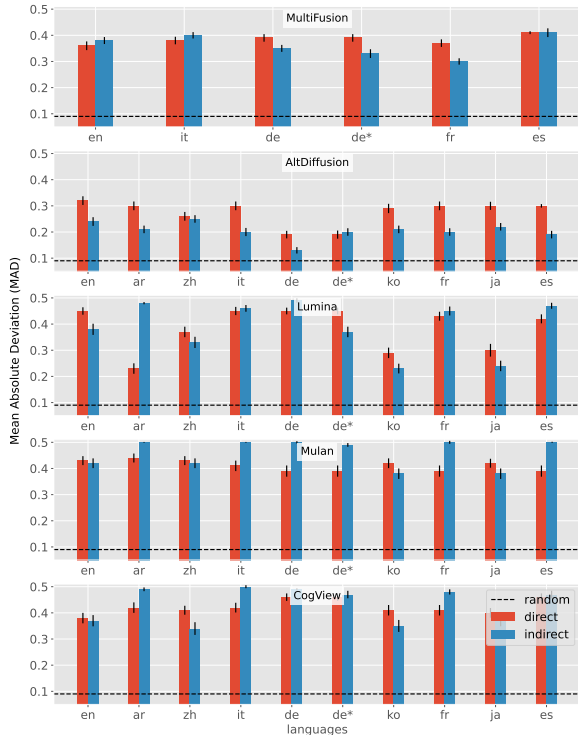
Figure 5: Occupation-gender bias results on MAGBIG for five multilingual T2I models. Red bars are images with direct prompts, \mathcal{I}_d , and blue ones are with indirect prompts, \mathcal{I}_i . Gender bias is present for all models across all languages and prompts, particularly compared to a randomly biased model (dashed). Rewriting occupations into indirect descriptions often lowers the MAD, i.e. gender bias, but cannot remove it.
