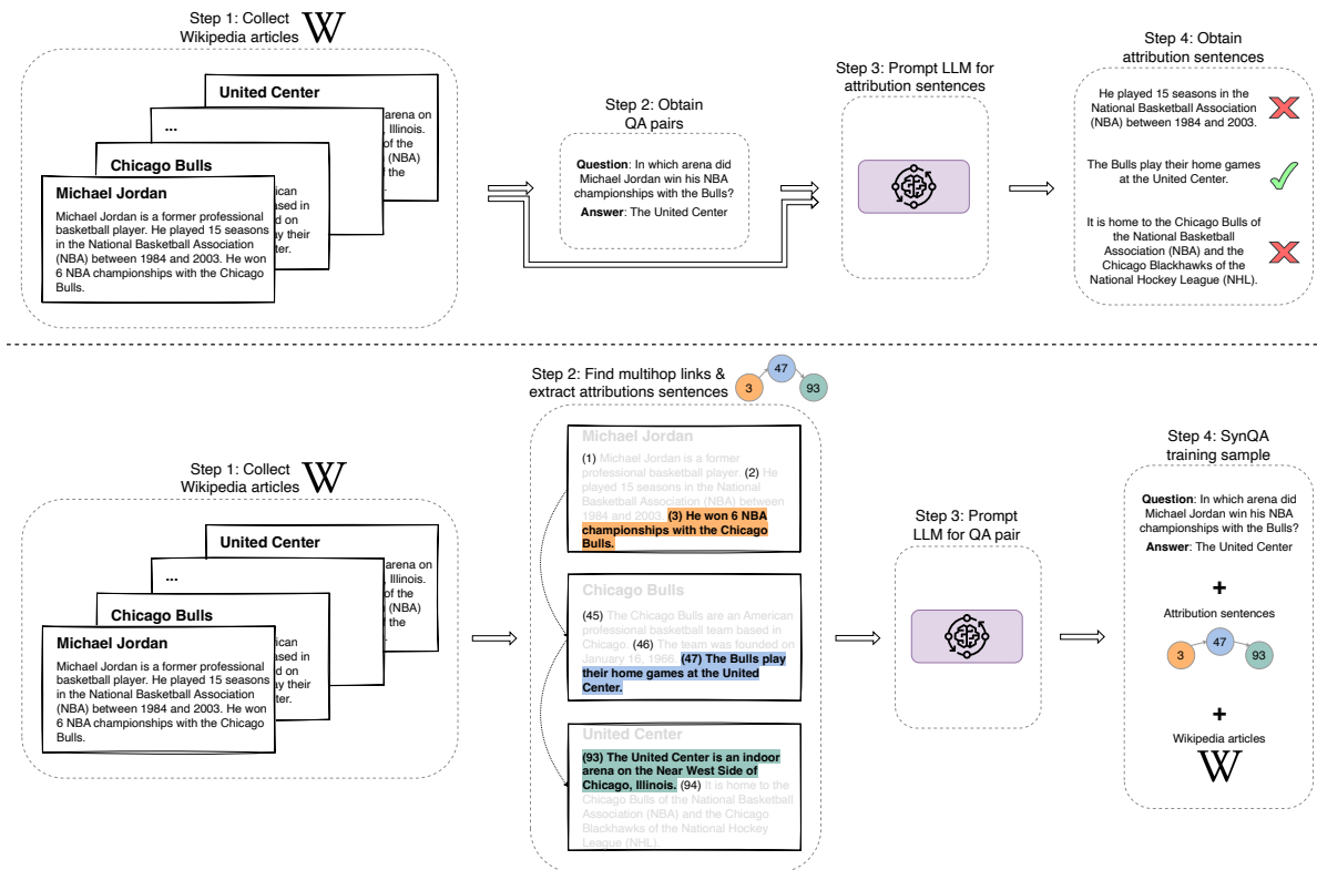
Figure 2: Top: The SYN-ATT baseline method for synthetic attribution data generation. Given context and question-answer pairs, we prompt an LLM to identify supporting sentences, which are then used to train a smaller attribution model. However, this discriminative approach may yield noisy training data as LLMs are less suited for classification tasks (see §3.3.1). Bottom: The SYNQA data generation pipeline leverages LLMs’ generative strengths through four steps: (1) collection of Wikipedia articles as source data; (2) extraction of context attributions by creating chains of sentences that form hops between articles; (3) generation of QA pairs by prompting an LLM with only these context attribution sentences; (4) compilation of the final training samples, each containing the generated QA pair, its context attributions, and the original articles enriched with related distractors.
