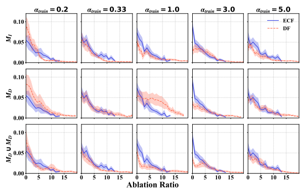
Figure 6: \Delta SP (y-axis) on ECF and DF for different \alpha_{train} configurations.
