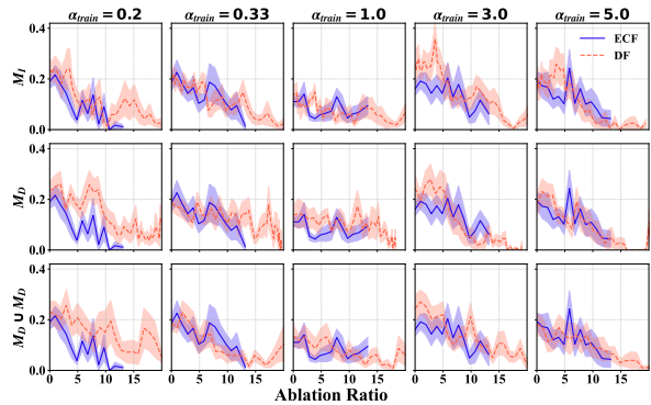
Figure 5: \Delta FPR (y-axis) on ECF and DF for different \alpha_{train} configurations.
