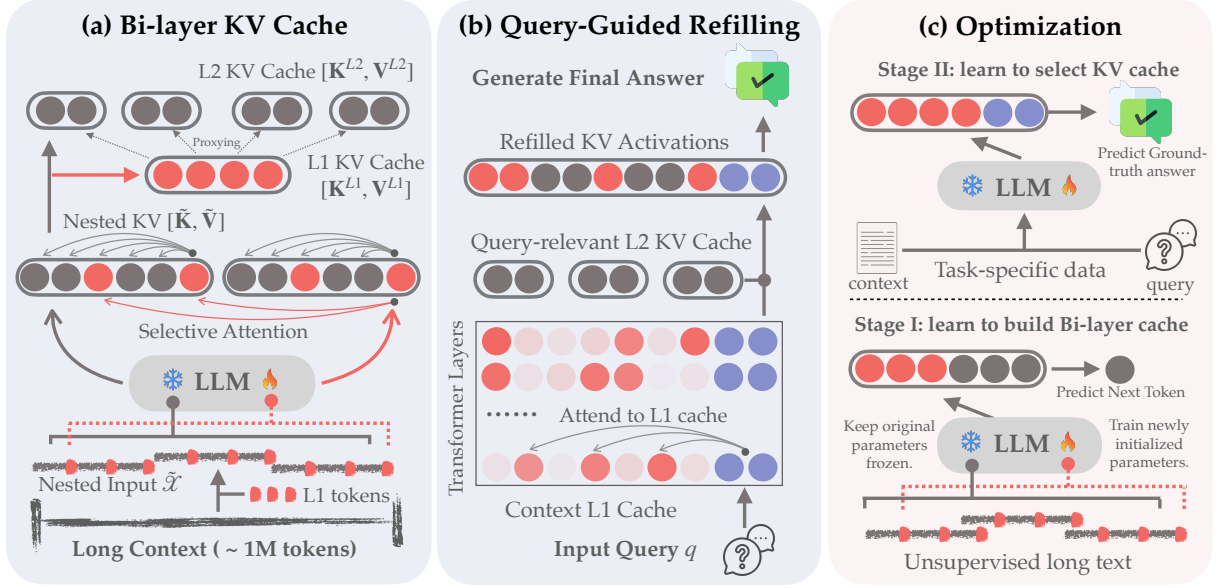
Figure 2: Overview of ACRE. (a) ACRE constructs the Bi-layer KV cache from a long context. (b) For an input query, ACRE refills the L1 KV cache with query-relevant entries from the L2 KV cache and decodes the final answer based on the refilled cache. (c) The two-stage optimization process used to train ACRE is illustrated.
