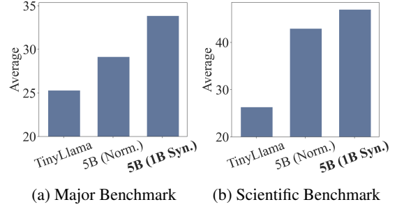
Figure 4: Performance of TinyLlama continually pre-trained on different corpora.
