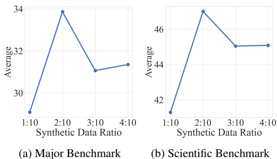
Figure 5: Performance of TinyLlama after training with different ratios of synthetic data.
