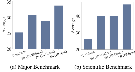
Figure 3: Performance of TinyLlama continually pre-trained on different open-source datasets.
