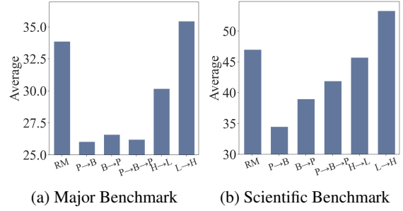
Figure 2: Performance of TinyLlama with different data curriculum methods. “RM” refers to the random mixing strategy. “P”, “B”, “H”, and “L” stand for “physics”, “biochemistry”, “high”, and “low”, respectively.
