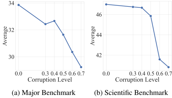
Figure 1: Performance of TinyLlama continually pre-trained on varying corruption levels of synthetic data.
