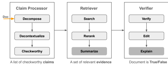
Figure 1: Fact-checker framework: claim processor, retriever, and verifier, with optional step of summarizing and explaining in gray.
