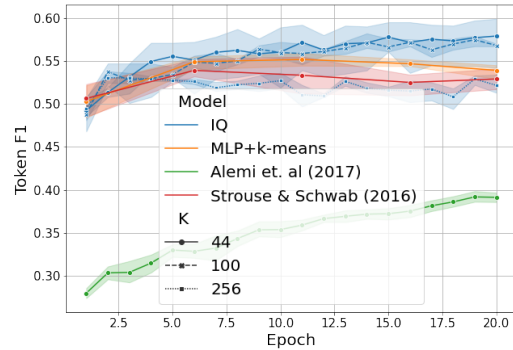
Figure 6: Token F1 convergence plot of various models on Flickr audio.
