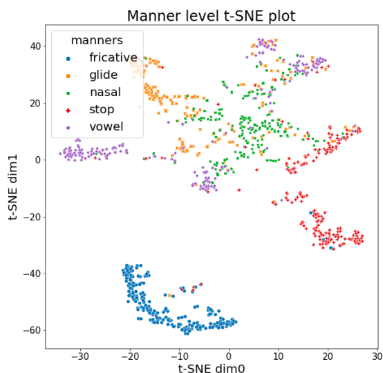
Figure 7: Manner-level t-SNE plots of phoneme clusters discovered by IQ with |\mathbb{Y}| = 161 and gold segmentation on Mboshi
