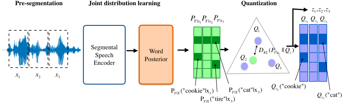
Figure 2: Network architecture of information quantizer
