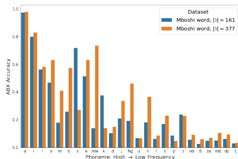
Figure 5: ABX phoneme identification accuracy vs phoneme frequency on the Mboshi dataset for IQ trained with vocabulary size 161 and 377.
