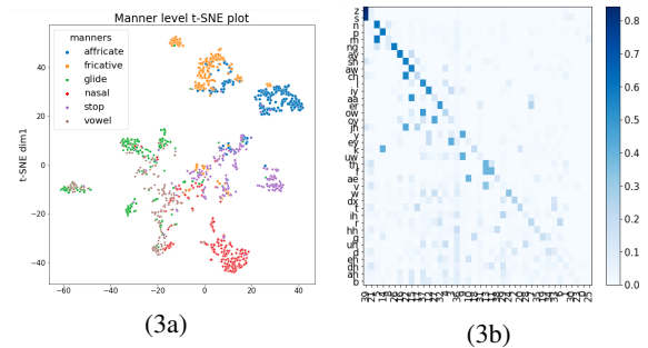
Figure 3: Left: Manner-level t-SNE plot by IQ with |\mathbb{Y}| = 824 and gold segmentation on TIMIT. Right: Distribution of codeword assignment for each phoneme by IQ with |\mathbb{Y}| = 824 and predicted segmentation on TIMIT. Each row of the plot is the empirical distribution for P_{\hat{Z}|Z}(\cdot|z) , 1 \leq z \leq K , where the phonemes are sorted top-to-bottom with decreasing \max_{z'} P_{\hat{Z}|Z}(z'|z) .
