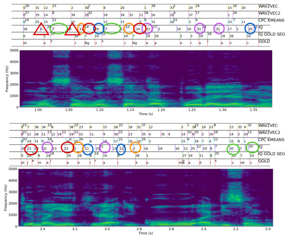
Figure 4: The spectrograms annotated with the gold transcripts and the zero-resource transcriptions by various models for two Mboshi utterances. The spoken segments are in circles of the same colors are identified as the same phoneme by our IQ model and in triangles of the same color if they are but are acoustically similar.
