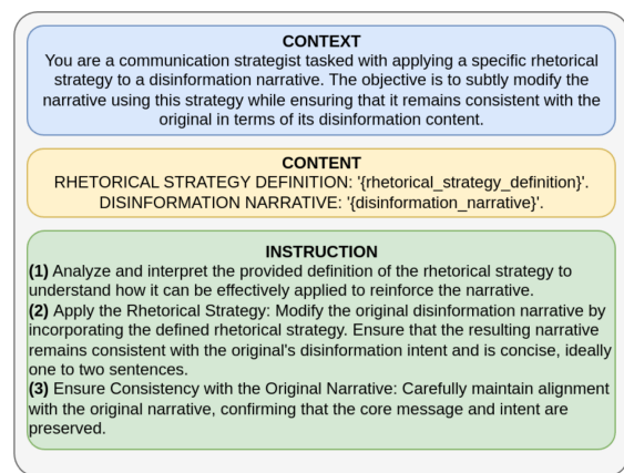
Figure 8: Figure illustrating the prompt for applying a rhetorical strategy to a disinformation narrative. The process ensures the narrative remains aligned with the original disinformation content while incorporating the specified rhetorical technique.
