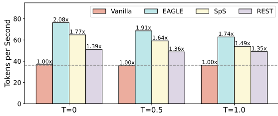
Figure 6: Speedup comparison of various methods on Spec-Bench at different temperatures. The speedup effect diminishes as the sampling temperature increases.
