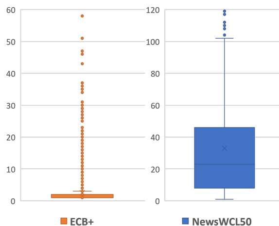
Figure 3: Difference in the size of coreference chains between ECB+ and NewsWCL50: ECB+ focuses on annotating some coreferential cases of strict identity relations whereas NewsWCL50 aims at covering all coreferential mentions with diverse identity relations.
