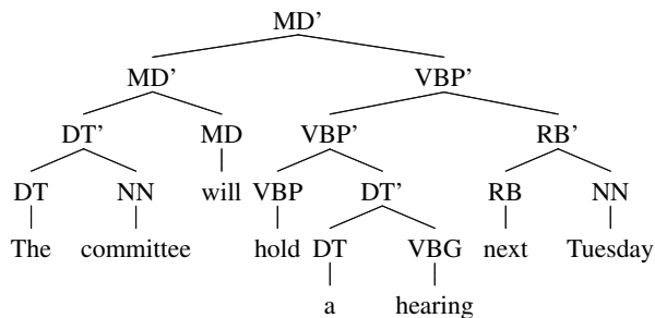
Figure 1: Example LSVM- G_x parse
