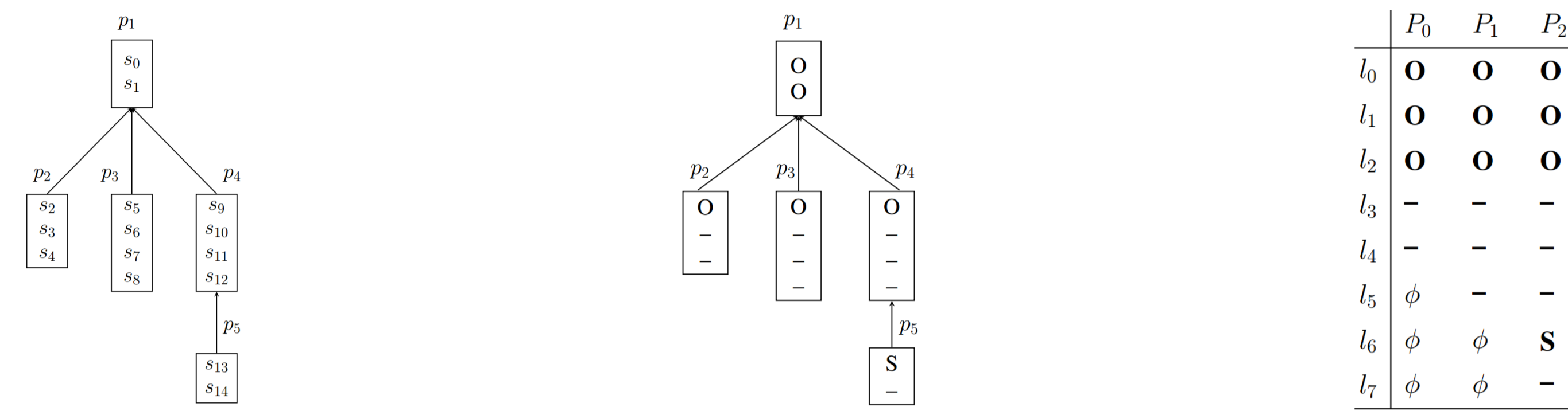
(a) Thread structure of a conversation (b) Entity role transition (c) 2D role transition matrix
