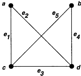
Figure 2: Simple graph with vertex cover \{c, d\} .
