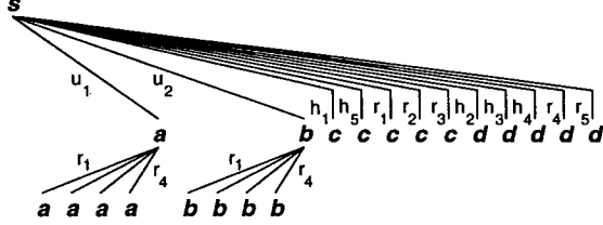
Figure 4: Encoding a solution to the vertex cover problem from Fig. 2.
