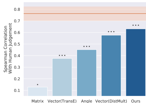
Figure 2: Spearman correlations between human judgment and models’ outputs. The inter-subject correlation is also shown as a horizontal line with its standard deviation as an error band. Our model shows the strongest positive correlation with human judgment, and, in other words, the smallest margin with human inter-subject agreement. Significance: ***/**/* := p < .001/.01/.05 .
