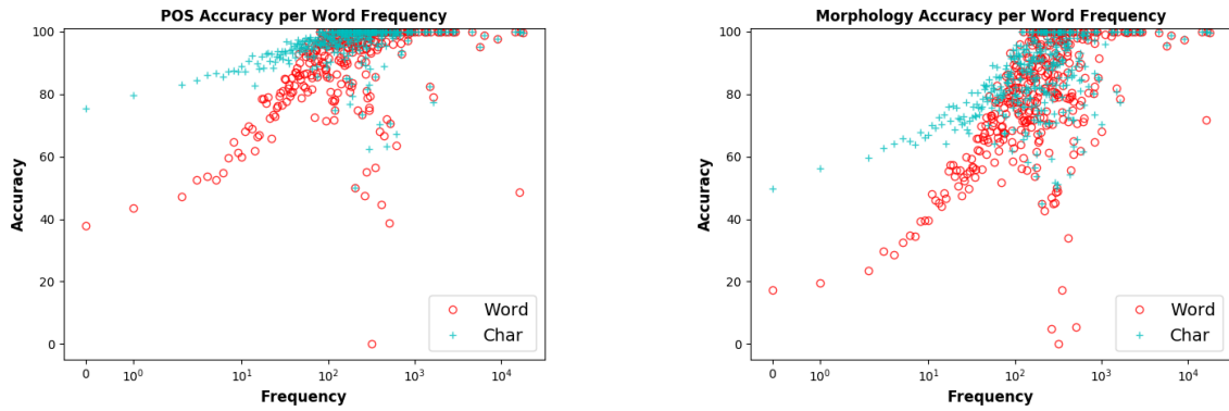
Figure 2: POS and morphological tagging accuracy of word-based and character-based models per word frequency in the training data. Best viewed in color.
