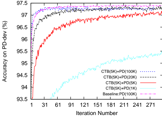
Figure 5: Accuracy on PD-dev with different weighting settings.
