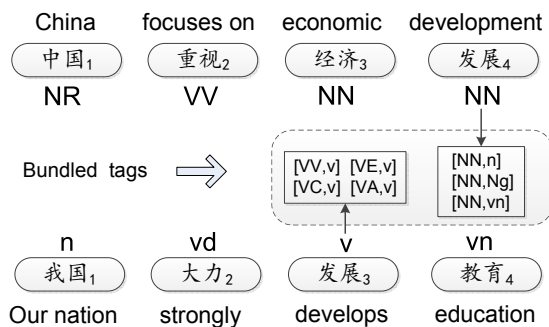
Figure 1: An example to illustrate the annotation differences between CTB (above) and PD (below), and how to transform a one-side tag into a set of bundled tags. “ NN ” and “ n ” represent nouns; “ VV ” and “ v ” represent verbs.
