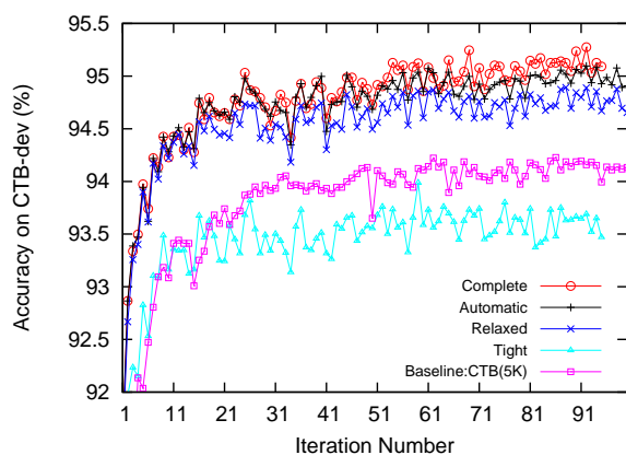
Figure 3: Accuracy on CTB -dev regarding to mapping functions.
