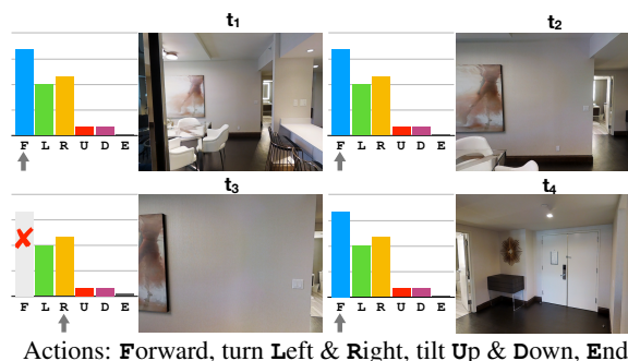
Figure 1: Navigating without vision leads to sensible navigation trajectories in response to commands like “walk past the bar and turn right”. At t_3 , “forward” is unavailable as the agent would collide with the wall.
