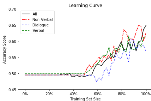
Figure 2: Learning curves (averaged 5-fold cross validation) for each modality using random forest (general truth/lie scenario)
