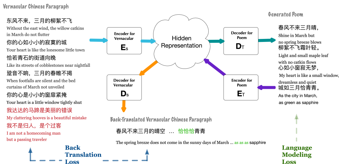
Figure 1: An example of the training procedures of our model. Here we depict two procedures, namely back translation and language modeling. Back translation has two paths, namely E_S \rightarrow D_T \rightarrow E_T \rightarrow D_S and D_T \rightarrow E_S \rightarrow D_S \rightarrow E_T . Language modeling also has two paths, namely E_T \rightarrow D_T and E_S \rightarrow D_S . Figure 1 shows only the former one for each training procedure.
