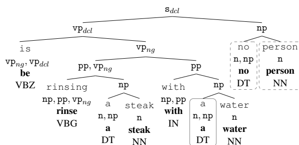
Figure 7: The corrected version of the CCG term of Figure 6, with inserted and decomposed terms.
