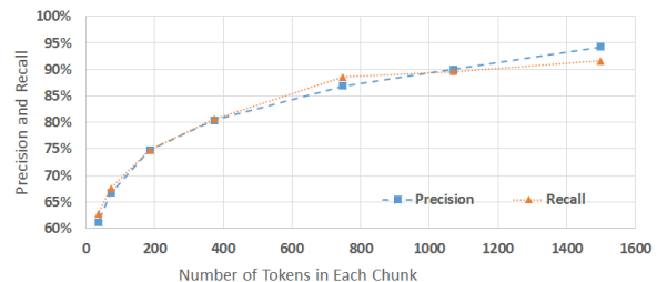
Figure 2: Effects of Chunk Size on Translationese Detection Accuracy 2
