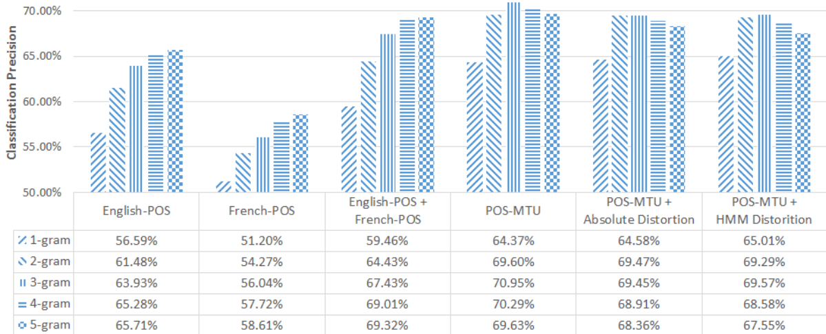
Figure 4: Sentence level translation direction detection precision using different features with n-gram lengths of 1 through 5.
