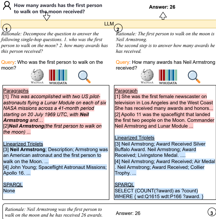
Figure 3: The illustration of DETLLM to instruct LLMs for addressing multi-source multi-hop questions.
