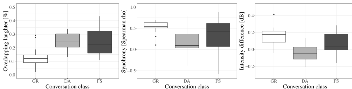
Figure 2: The results of the investigated entrainment measures, with respect to the considered conversation classes: overlapping laughter (left panel), synchrony (middle panel) and form-related measure (right panel). The horizontal line represents the median value, the hinges of the boxes the first and third quartiles, and the whiskers going up to 1.5 \cdot \text{IQR} (inter-quartile range) from the hinges.
