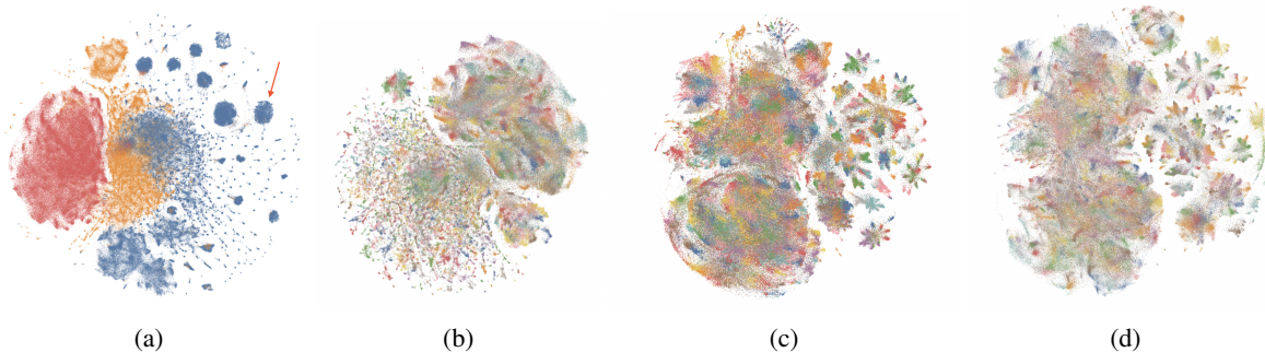
Figure 1: TSNE visualizations showing the progression of the GPT4All train set. Panel (a) shows the original uncurated data. The red arrow denotes a region of highly homogeneous prompt-response pairs. The coloring denotes which open dataset contributed the prompt. Panel (b) shows the original GPT4All data after curation. This panel, as well as panels (c) and (d) are 10 colored by topic, which Atlas automatically extracts. Notice that the large homogeneous prompt-response blobs no longer appear. Panel (c) shows the GPT4All-J dataset. The "starburst" clusters introduced on the right side of the panel correspond to the newly added creative data. Panel (d) shows the final GPT4All-snoozy dataset. All datasets have been released to the public, and can be interactively explored online. In the web version of this article, you can click on a panel to be taken to its interactive visualization.
