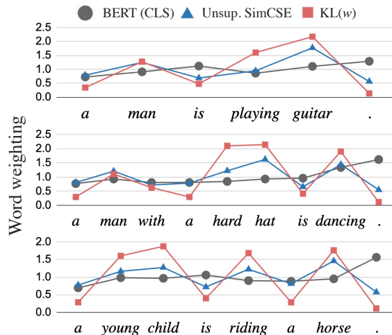
Figure 3: Sentence-level examples of the word weighting of BERT (CLS) and Unsupervised SimCSE-BERT using IG. Same as IG, KL(w) is normalized so that the sum of KL(w) becomes the sentence length for visibility. For words like “ man ”, “ child ”, “ guitar ”, “ is ”, “ hat ”, “ horse ” and “ . ” the word weightings of the contrastive fine-tuned model (▲) are closer to KL(w) (■) than the pre-trained model (●), which means that contrastive fine-tuning induces word weighting by KL(w) .
