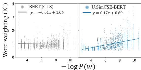
Figure 6: Linear regression plots between -\log P(w) and the word weighting of BERT (CLS) (left) and Un-supervised (U.) SimCSE-BERT (right) using IG. We plotted subsampled 3000 tokens from the tokens with the top 99.5% of small KL values for visibility.
