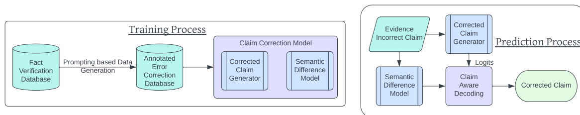
Figure 1: Full Description of the SciFix system. During training a fact verification database is converted to a well annotated error correction database using Prompting with LLMs, this database is used to train a Seq2Seq correction LM and a Seq2Label Semantic Difference Model. During prediction the semantic difference model helps guide the generative model using claim aware decoding to generate the corrected claim
