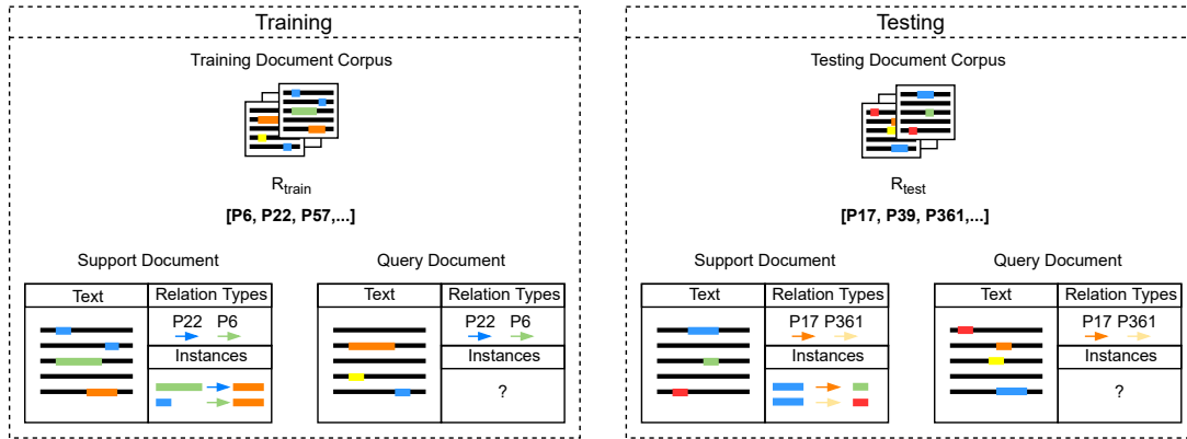
Figure 1: Illustration of an episode in the Few-Shot Document-Level Relation Extraction setting. Given a support document with annotated relation instances, the task is to return all instances of the same relation types for the query document. During testing a different corpus of documents, as well as a different set of relation types are used than during training.
