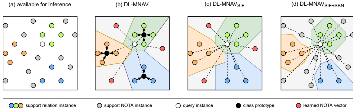
Figure 2: Embedding space illustration of the different models used for evaluation at inference time . Shown in (a) are all data points available from support documents, as well as the query instance. Class prototypes in (b) are computed as mean of support relation instances. Learned NOTA vectors, shown in red, are not based on support NOTA instances but learned during training and do not change based on the support document. Dotted lines indicate distances affecting the classification of the query instance, shown in white. Background colors illustrate approximate classification boundaries. For the baseline model (5.1.1), decision boundaries are the same as in (d).
