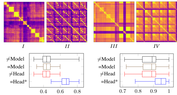
(a) Constituency Similarity (b) Dependency Similarity
