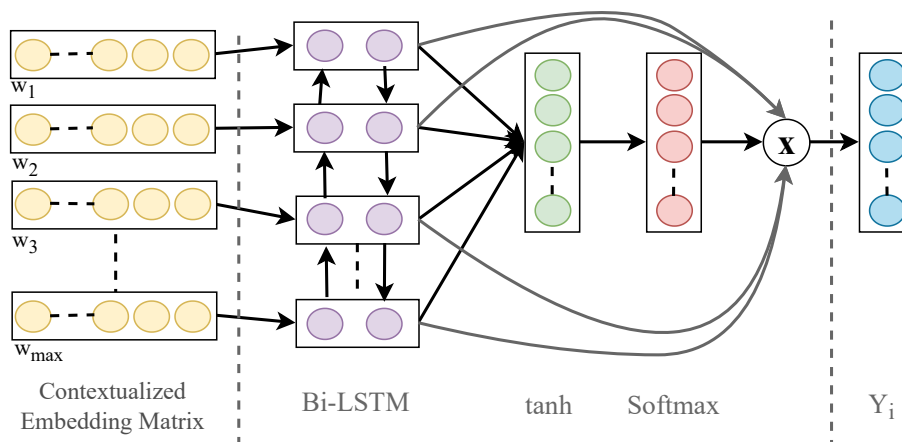
Figure 2: Architectural illustration of the attention mechanism used in the proposed model
