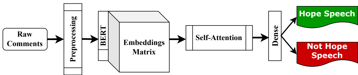
Figure 1: Flowchart illustration of the proposed model for Hope Speech classification.
