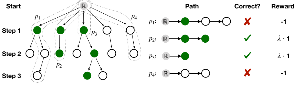
Figure 2: An example of our RLHR approach with M = 4 . Green circles are the ground truth labels. p_1, p_2, p_3 , and p_4 are four sampled deduction paths, where p_3 ends before it arrives at a leaf label.
