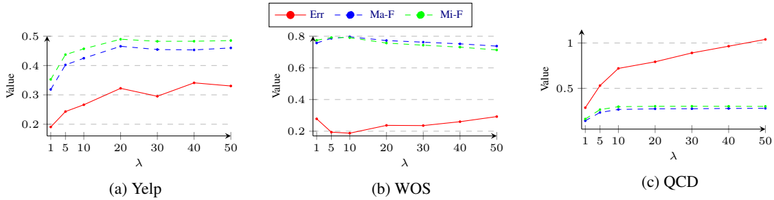
Figure 3: Influence of \lambda on RLHR approach with BERT. Err, Ma-F and Mi-F denote logical error rate, Macro-F1 and Micro-F1 respectively.
