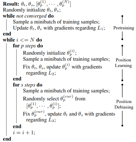
Algorithm 1: Alternating Adversarial Learning
