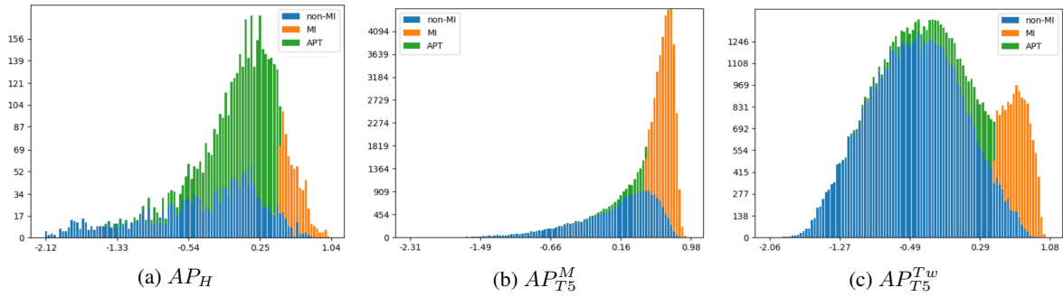
Figure 2: BLEURT distributions on adversarial datasets. All figures divide the range of observed scores into 100 bins. Note that APT sentence pairs are also MI , whereas those labeled ‘ MI ’ are not APT .
