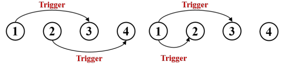
(a) (1 \xrightarrow{l_t} 3) and (2 \xrightarrow{l_t} 4) . (b) (1 \xrightarrow{l_t} 2) and (1 \xrightarrow{l_t} 3) .
