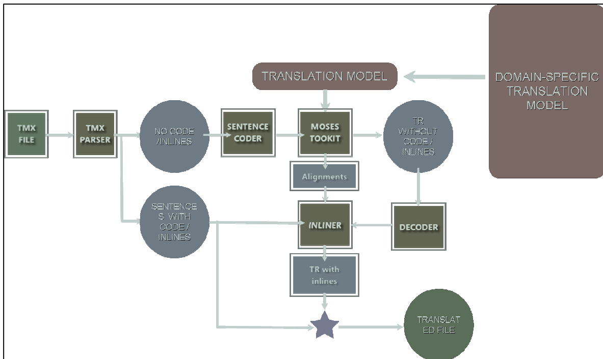
Figure 3. PangeaMT Translation Model
