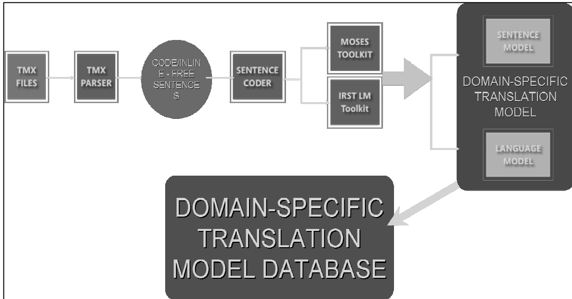
Figure 1. PangeaMT Training Model
