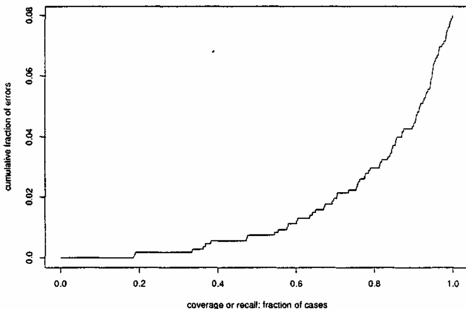
Figure 4. The horizontal axis shows coverage while the vertical scale shows error rate. Note that the error rate increases very quickly with small increases in coverage, because most of the errors result when there is very little information to go on.
