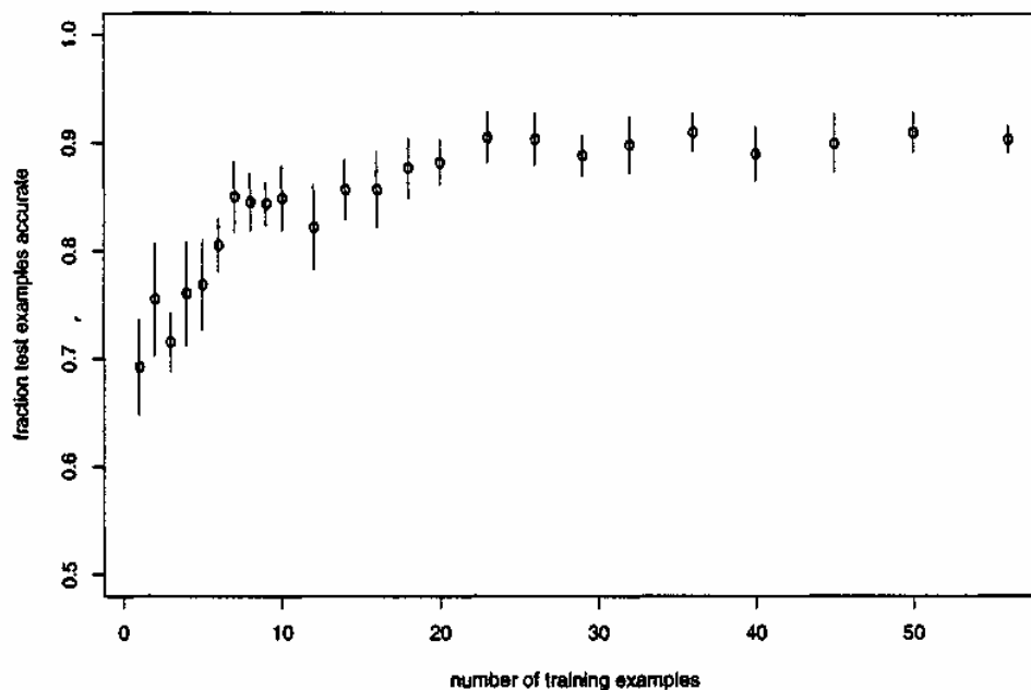
Figure 3. The horizontal axis shows the size of the training set, while the vertical scale shows performance (percent correct, averaged over 90 instances times two senses times six polysemous words). Note that very small training sets perform remarkably well; just 3 exemplars are sufficient to achieve 75%. Nevertheless, it helps to use larger training sets, up to about 50 or 60 exemplars when performance reaches asymptote.
