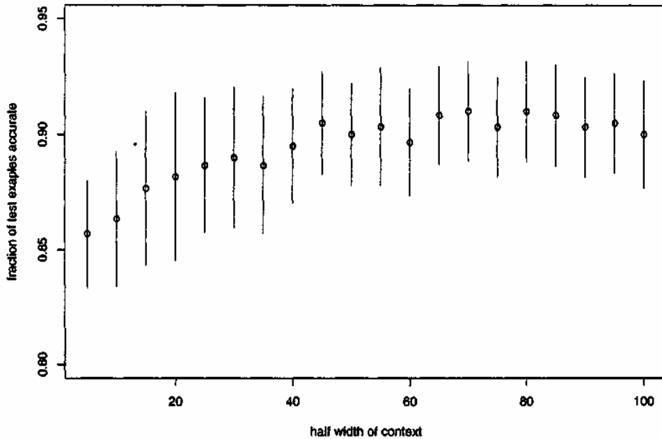
Figure 2. The horizontal axis shows the size of the context, as in Figure 1. The vertical axis shows performance (percent correct), computed over a context of 2d-1 words, from -d to d (but excluding 0). Note that performance rises very rapidly at first and reaches an asymptote at about 50 words.
