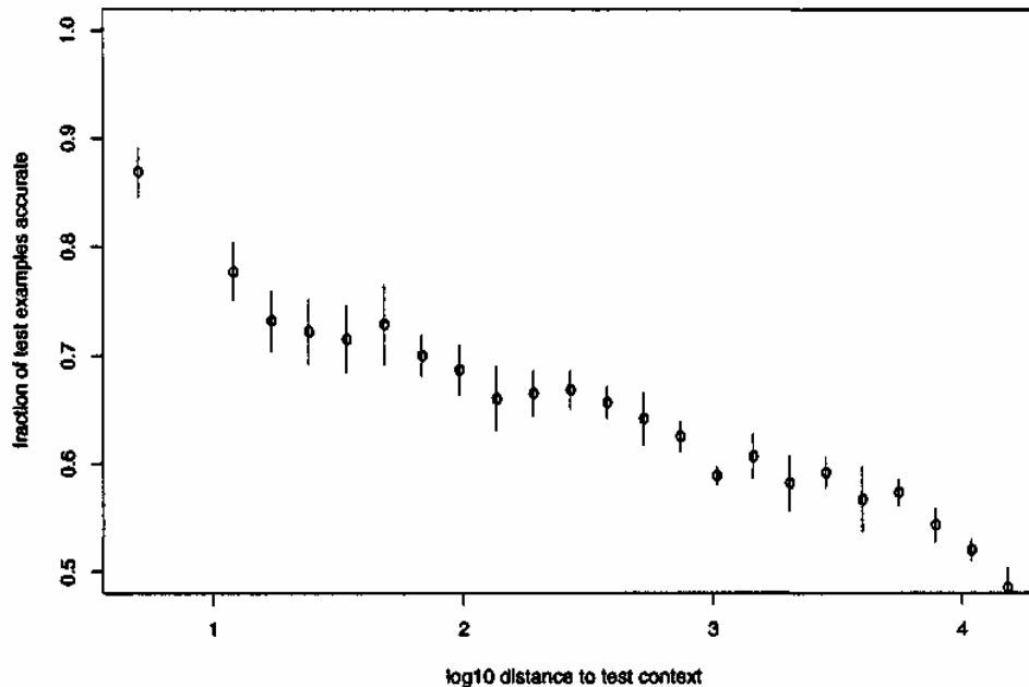
Figure 1. The horizontal axis d shows the size of the context as a distance (in words) from the polysemous word in question. The vertical scale shows disambiguation performance (percent correct), computed over a context of ten words at the distance specified by the horizontal axis: [-d-5,-d] and [d, d+5] . Vertical lines indicate means and standard deviations computed over a group of 90 instances times six polysemous words times two senses. Note that performance remains significantly above chance (50%) out to 10,000 words away from the polysemous word.
